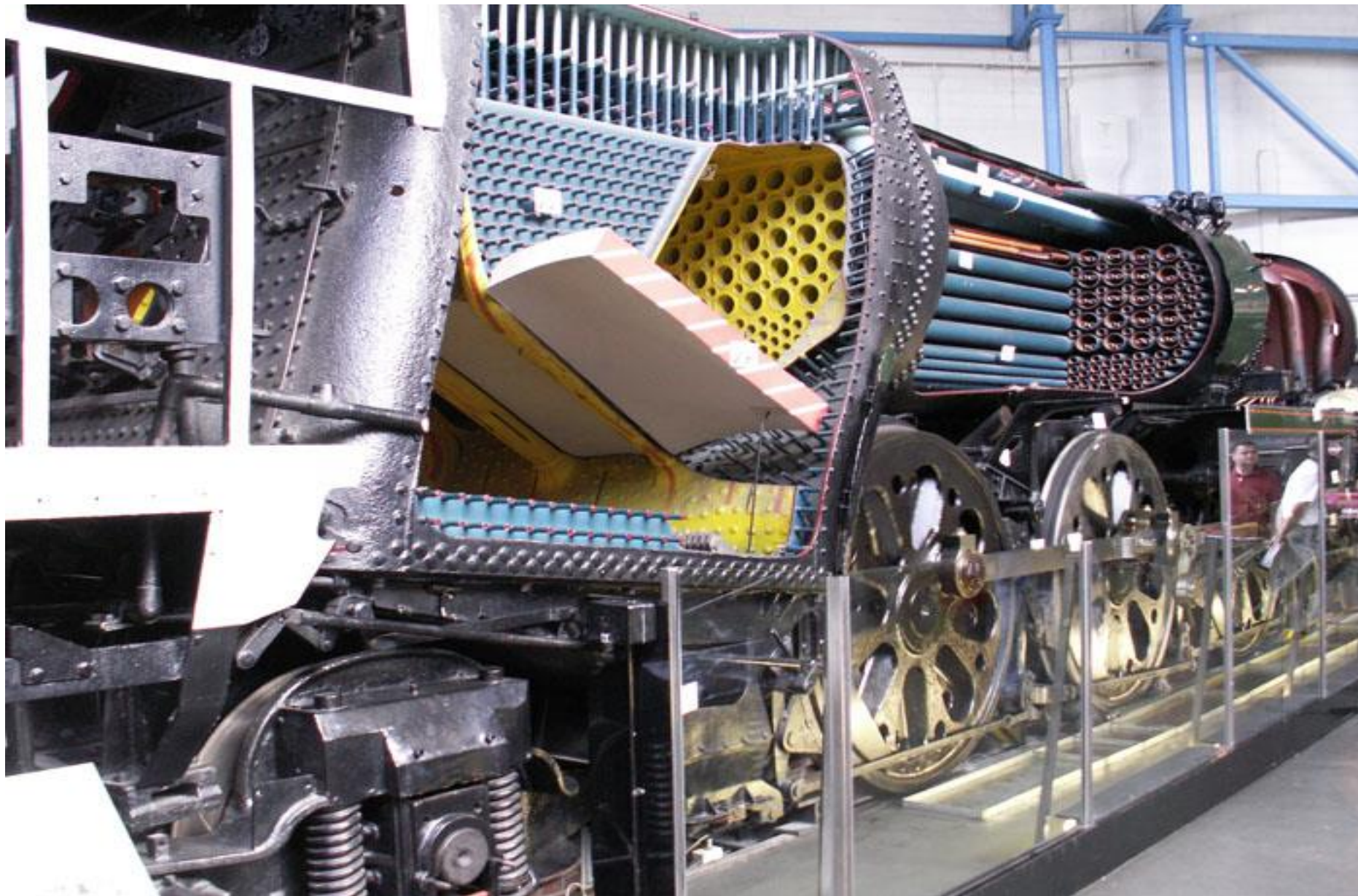
Merchant navy class boiler showing the sectioned firebox
